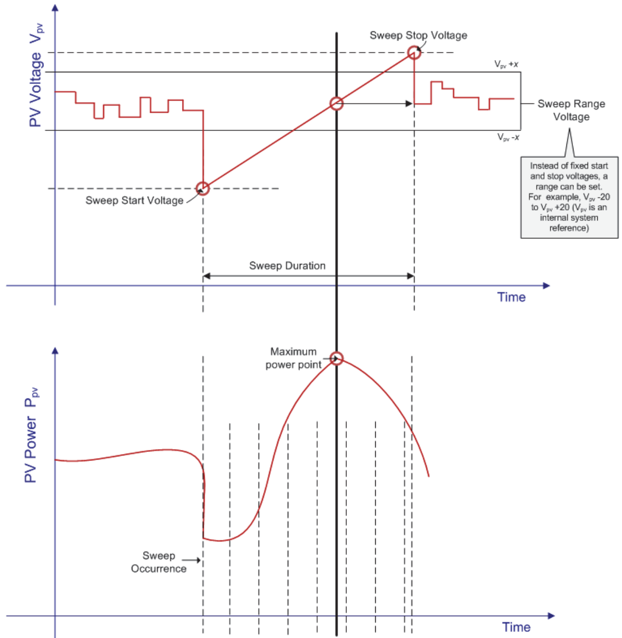
Figure 10 Sweep settings
