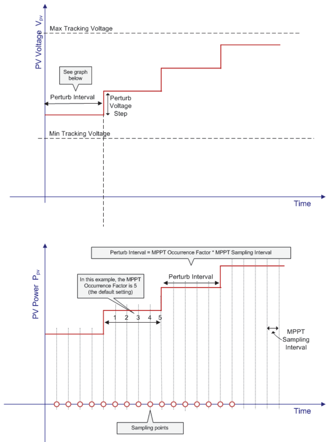
Figure 5 MPPT perturbations
